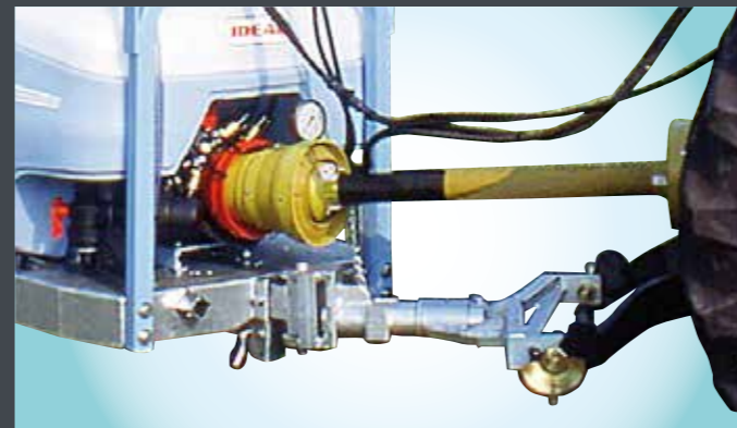
Timone articolato / Tracker drawbar / Attelage articulé / Gelenkdeichsel / Tiro articulado
